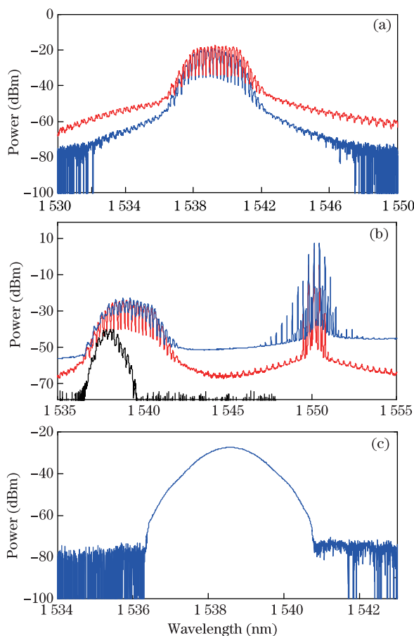
Fig. 4. (Color online) Optical spectra: probe before (red line) and after (blue line) 3 nm optical BPF; (b) probe and pump before (red line) and after (blue line) SOA and after the waveshaper (black line). (c) The frequency curve of the offset filter.
