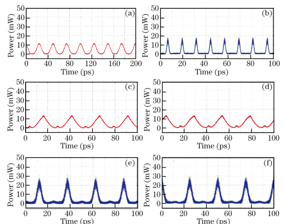
Fig. 3. Waveforms of (a) 40-GHz pump signal, (b) 80-GBd OTDM-DQPSK signal, (c) mixed signal of pump and probe before SOA while demultiplexing channel 1, and (d) signal of pump and probe before SOA while demultiplexing channel 2. Eye diagrams of the demultiplexed channels (e) 1 and (f) 2.
