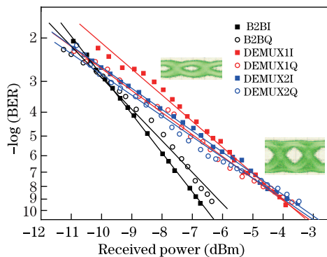
Fig. 5. (Color online) BER performance for B2B (black) operation and channels 1 (red) and 2 (blue). DEMUX: demultiplexed channel.
