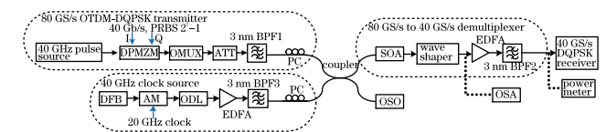
Fig. 2. Experimental setup. (DPMZM: dual-parallel MZM; ATT: attenuator; DFB: distributed feedback laser; OSO: optical sampling oscilloscope; OSA: optical spectrum analyzer).
